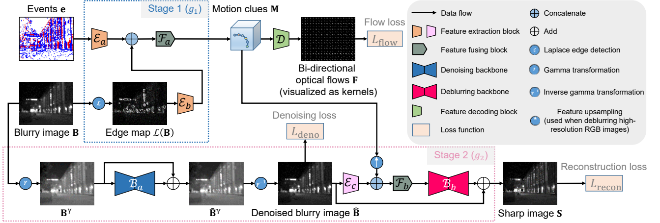
Fig. 2 We design a motion-aware neural network tailored to our unified two-stage framework (Figure 1 (right)). In the first stage, it extracts features from the edge map of the APS image and corresponding events jointly to obtain both spatial and temporal information about motion, and encodes the information into high-fidelity motion clues by explicitly using bi-directional optical flows to supervise this process in the latent space. In the second stage, it adopts a denoising module to perform blind noise suppression in the image domain to avoid ringing artifacts, and reconstructs the sharp image under the guidance of motion clues.
