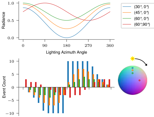
Figure 4. Given 4 points with coordinates (elevation angle \theta , azimuth angle \phi ) of blue: (30^\circ, 0^\circ) , orange: (45^\circ, 0^\circ) , green: (60^\circ, 0^\circ) , and red: (60^\circ, 90^\circ) on a sphere, and a light source rotating in a clockwise circle, the radiance changes (top) and events triggered (bottom) of the 4 points w.r.t. light direction changing are plotted. The bottom part shows event number determines the normal elevation angle (comparing blue, orange, and green points), while the zero-crossing point determines the normal azimuth angle (comparing green and red points).
