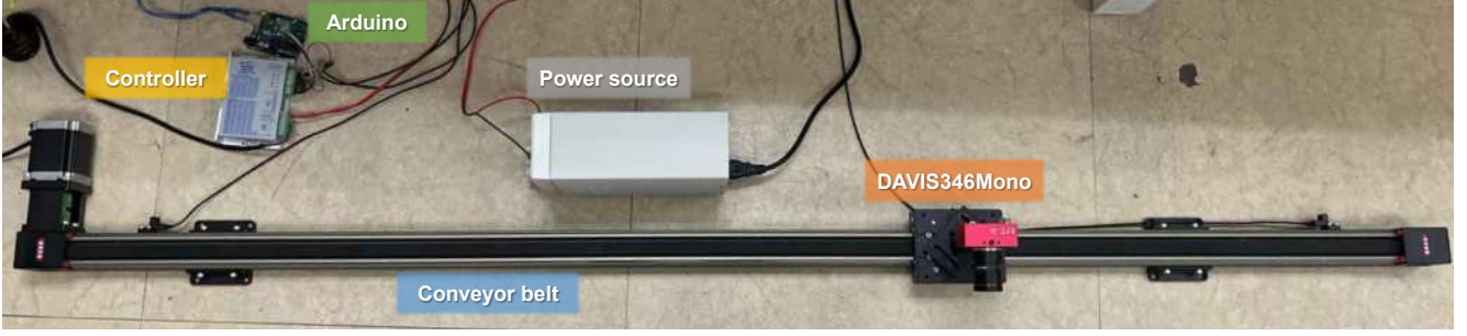
Figure 8. Illustration of the experimental setup for constant speed using a conveyor belt. The Arduino sends signals to the controller at a constant frequency, and the controller controls the speed and the direction of the belt at a constant speed.
