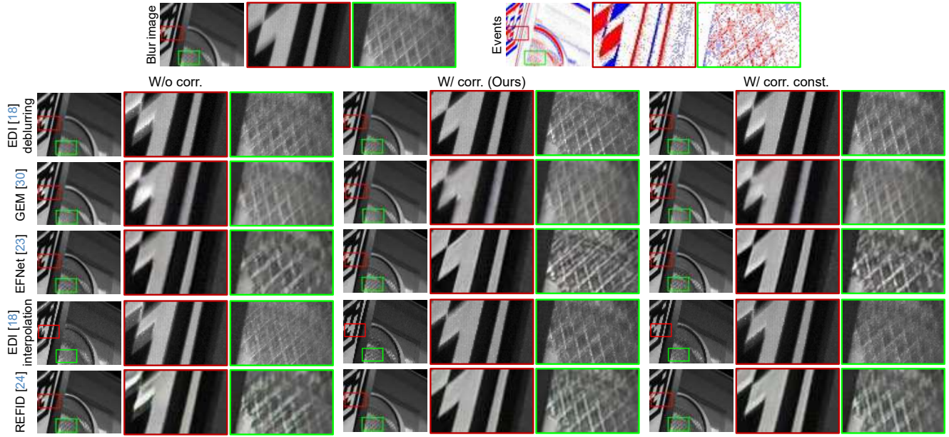
Figure 18. The qualitative comparison on real data. We correct the latency of events by constant latency correction (“W/ corr. Const.”) and spatially-varying latency correction (“W/ corr.”). All the methods are tested with the same input. The proposed event latency correction method effectively mitigates latency effects, improving the performance of existing deblurring and interpolation techniques in low-light conditions.
