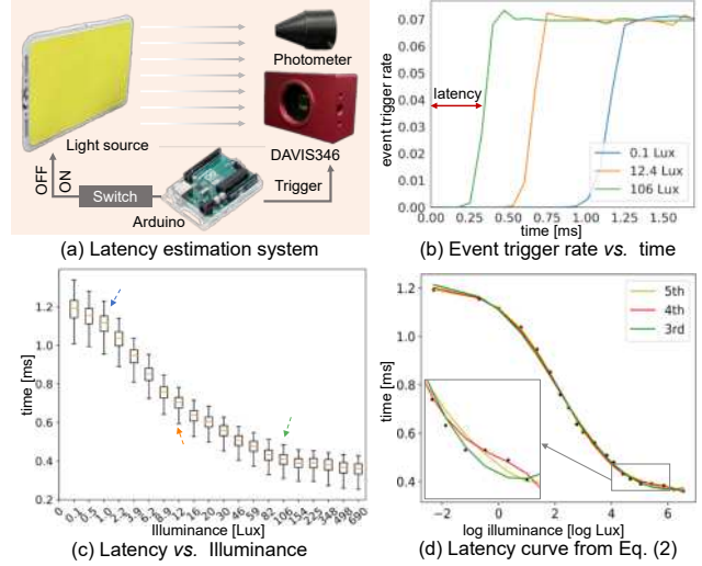
Figure 3. Estimation of latency-illuminance curve. (a) A system designed to investigate the relationship between illuminance levels and latency, approximated using an K -th order polynomial. (b) The comparison of event triggering rate under three varied lighting conditions. It is approximated by the first 1% OFF events in our experiments. (c) Estimated latency under controlled lighting, highlighting increased latency with diminishing light. (d) Results of the polynomial approximation.
