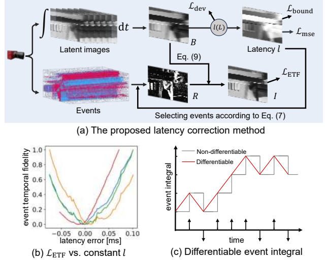
Figure 2. Illustration of the proposed latency correction method. (a) The pipeline of the proposed method, which takes synchronized blurry image B and events as input, and output the latency l by polynomial function l(L) . (b) The value of the proposed event temporal fidelity (ETF) \mathcal{L}_{\text{ETF}} decreases as the estimated latency approaches ground-truth latency, which validates the efficacy of ETF as an objective. (c) Latency-differentiable reformulation of event integration, enabling gradient-based optimization.
