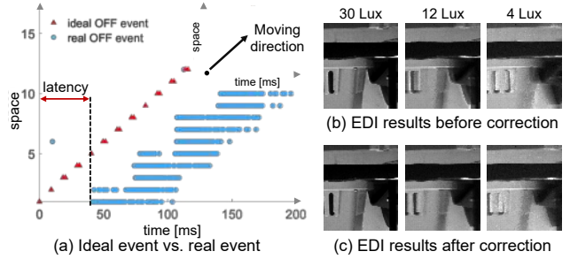
Figure 1. Illustration of latency in an event camera, and its influence on an event-guided deblurring algorithm. (a) The aerial view of ideal vs. real events triggered by a black point moving upwards on a white background, where the real events are captured in low-light conditions (below 0.1 Lux). (b) Deblurring results using the Event-based Double Integral (EDI) [19] method, guided by events captured under different illumination conditions. (c) Improved deblurring results from EDI [19] using event with latency corrected by the proposed method.
