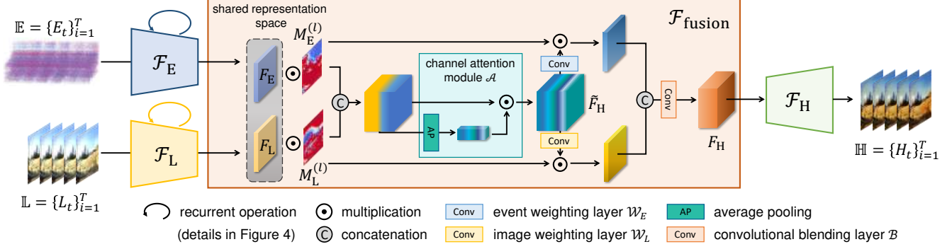
Figure 2. Overview of the proposed HDRev-Net. For multimodal representation alignment, the hybrid inputs of stacked events \mathbb{E} and LDR frames \mathbb{L} are mapped onto a shared representation space by the modality-specific encoders \mathcal{F}_E, \mathcal{F}_L , in which recurrent connections are applied for temporal context encoding. Under the guidance of confidence masks M_E and M_L extracted from \mathbb{E} and \mathbb{L} , respectively, their latent representations F_E, F_L are then integrated into a joint one F_H by the multimodal fusion module \mathcal{F}_{\text{fusion}} . The HDR decoder \mathcal{F}_H decodes F_H into HDR frame sequence \mathbb{H} eventually.
