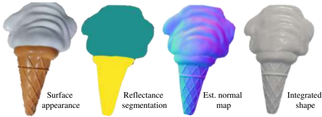
Figure 2: Our method can be applied to spatially-varying general reflectance with given reflectance segmentation. The integrated shape of our normal estimation is consistent with the surface appearance.
