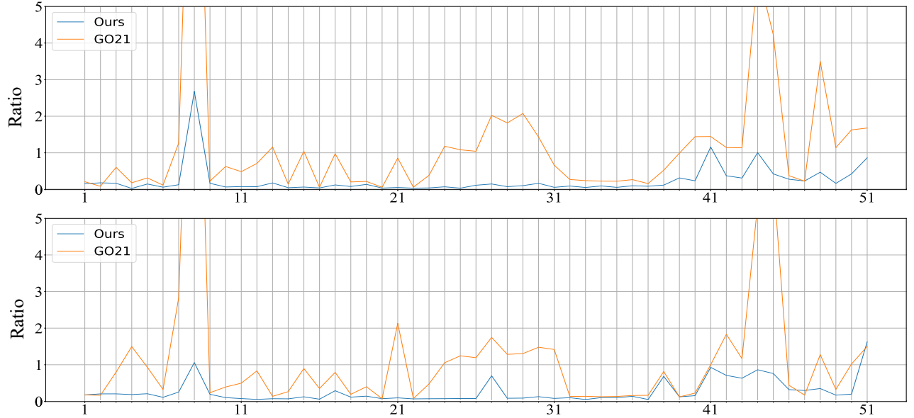
Figure 5: Results of predicted equivalent light intensities for diverse materials [Dupuy and Jakob, 2018] on SPHERE (upper part) and BUNNY (lower part) test dataset. The X-axis indicates indices of the materials. The predicted equivalent light intensities for each material are evaluated using the mean of “ratio” defined in Eq. (1).
