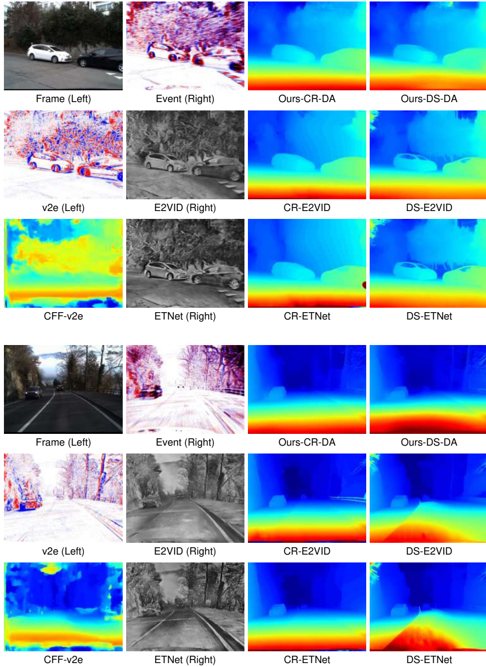
Figure 9: Qualitative comparison of our method and baselines. Our methods demonstrate better robustness.
