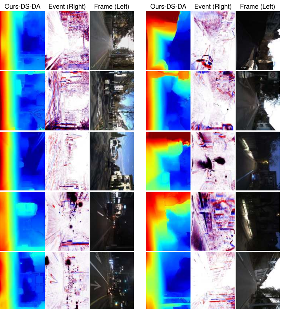
Figure 14: Results of our method in diverse scenarios.
