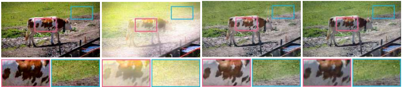
(l) MBLEN [8]
