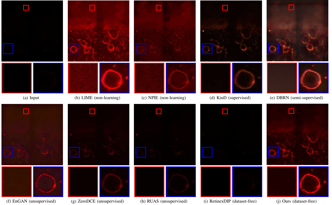
Fig. 10. Visual comparison of enhancement results on a fluorescent image. It can be seen that the performance of ZeroDCE, RUAS, and RetinexDIP is relatively poor. Although NPIE and EnGAN improve the contrast, they also greatly amplify the noise. KinD and DBRN can improve contrast while suppressing noise, but they also blur out some important details. In contrast, the proposed method can improve the contrast while preserving details during denoising.
