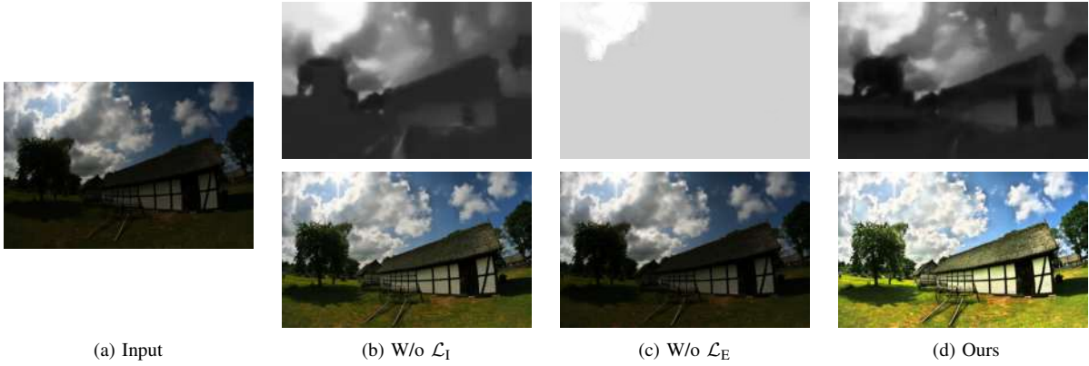
Fig. 9. Ablation study on the regularization loss. (b)-(d): Top: Illumination; Bottom: Output. As shown in (b), using a fixed \gamma instead of an adaptive one guided by \mathcal{L}_I produces unsatisfactory result and contrast. As shown in (c), without the intensity distribution regularization \mathcal{L}_E , \mathcal{G}_E outputs a trivial constant illumination map.
