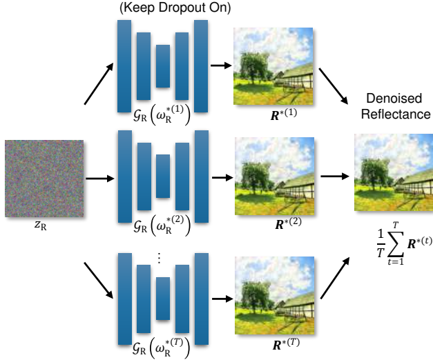
Fig. 4. Dropout ensemble for inference of G_R . Once G_R is sufficiently optimized, the denoised R is obtained by averaging over multiple R s produced by running G_R(\omega_R^*) T times with its nodes kept randomly dropped out.
