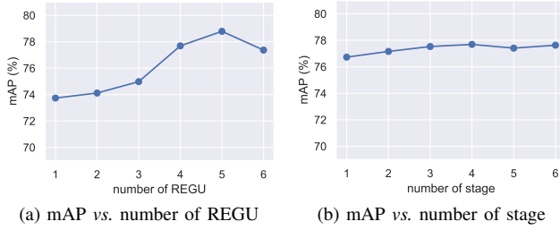
Fig. 8. Sensitivity studies on the hyper-parameters.
