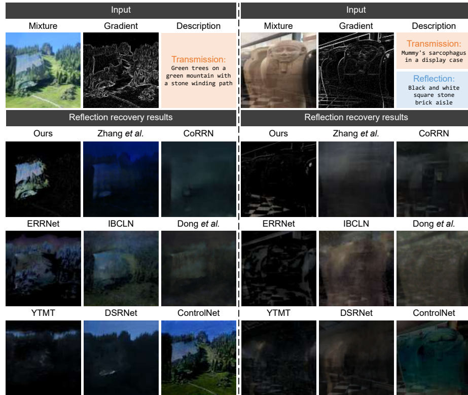
Fig. 8: Qualitative comparison of estimated reflection layers on real mixture images collected from the Internet, compared with several single-image methods [2, 9, 10, 12, 17, 21, 23] and a diffusion-based method ControlNet [22]. Please zoom in for details.
