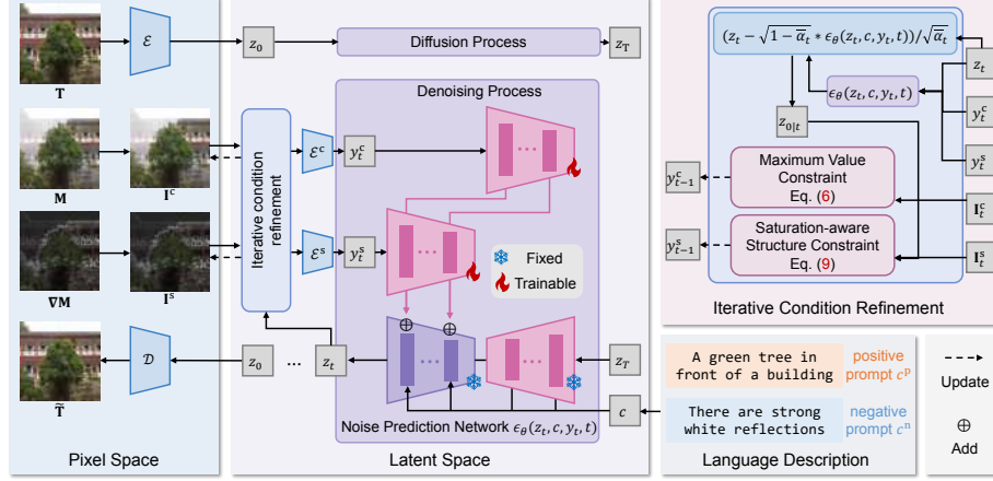
Fig. 2: Framework of the proposed language-based reflection removal diffusion model, which leverages language descriptions with the iterative condition refinement strategy and the multi-condition constraint mechanism to achieve faithful transmission recovery.
